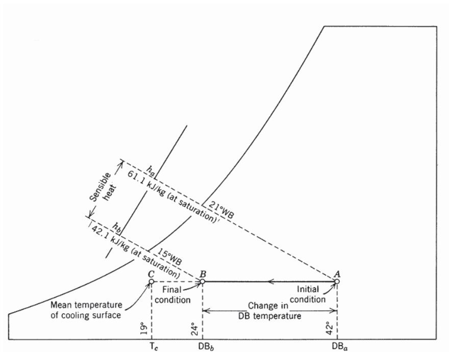
Gambar 4.9 Sketsa Proses Pendinginan Sensibel
