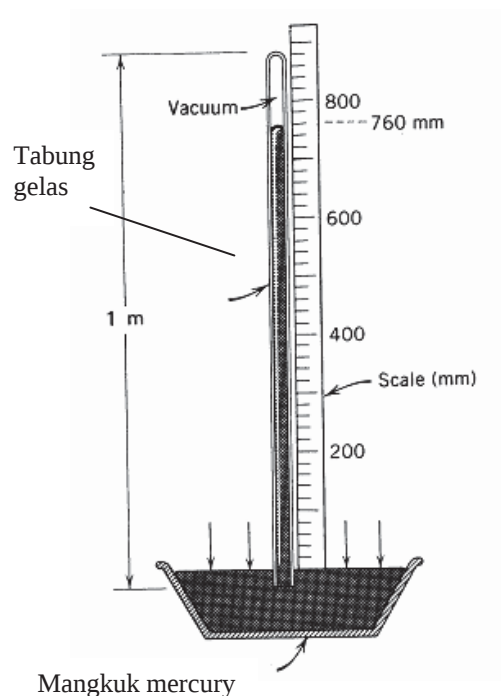
Gambar 2.6 Barometer mercury
