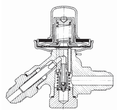
Gambar 9.3 Konstruksi automatic expansion valve
