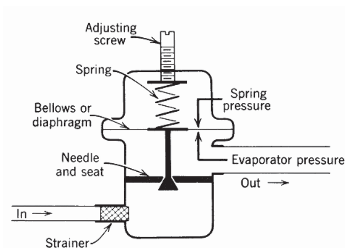
Gambar 9.2 Diagram skematik automatic expansion valve
