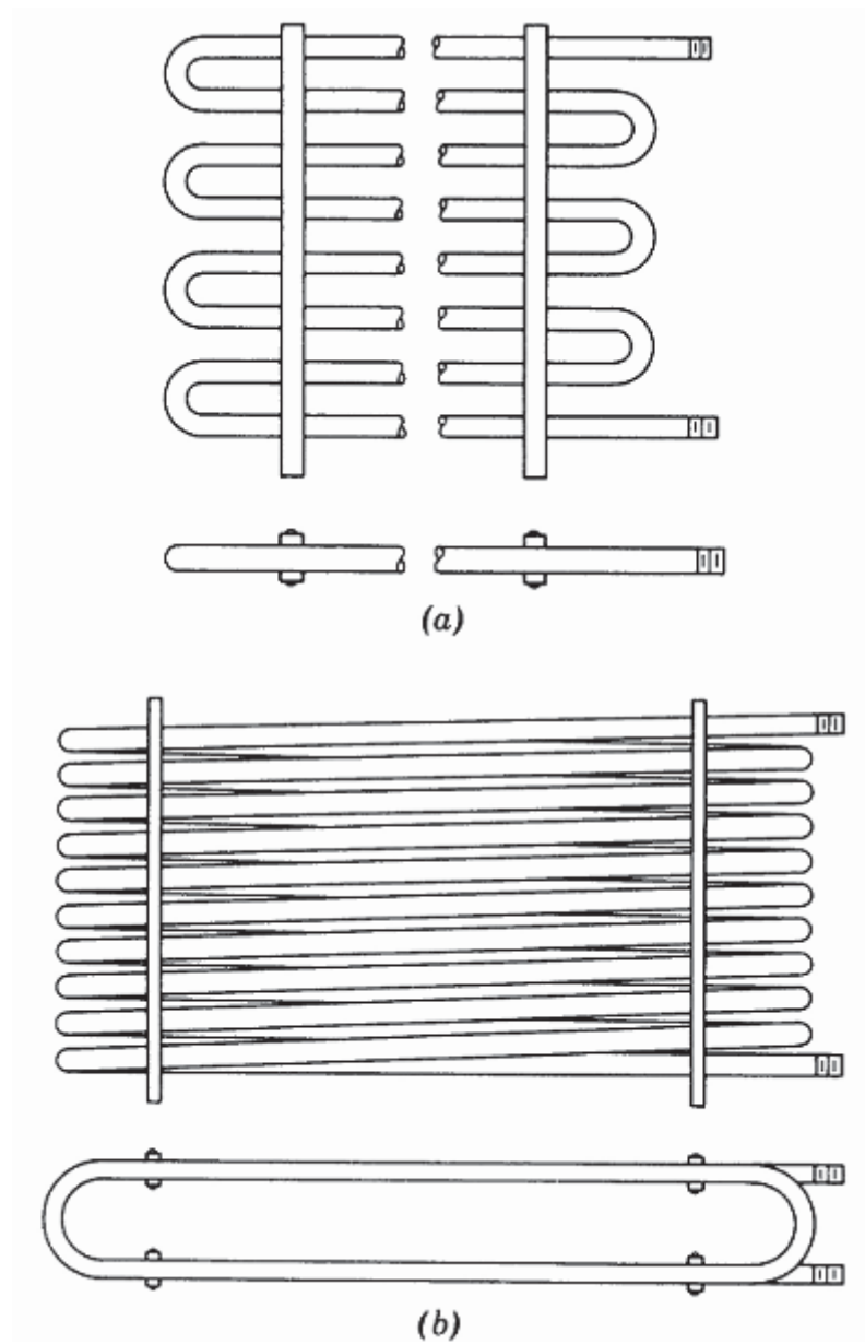
Gambar 8.1 Desain Evaporator Bare-tube. (a) Flat zigzag coil, (b) oval trombone coil
