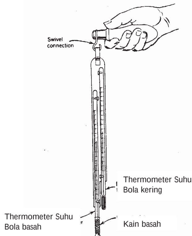
Gambar 3.10 Sling Psychrometer
