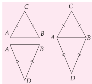
Gambar 8.8 Layang-layang ADBC
