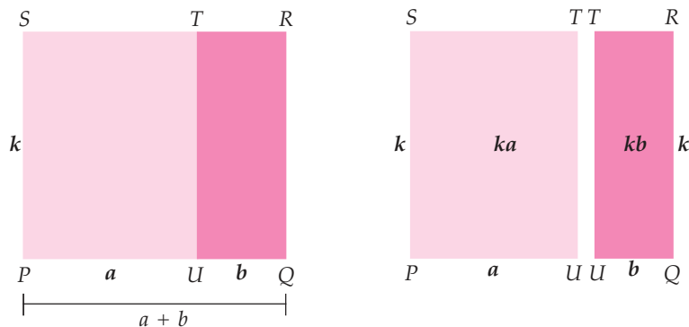
Gambar 2.1 \square PQRS
