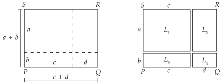
Gambar 2.2 \square PQRS
