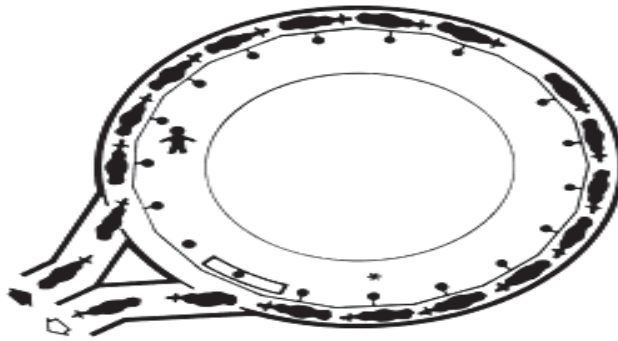
Gambar 22. Layout Mesin Perah Tipe Rotary Tandem
