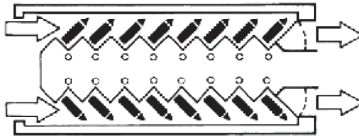
Gambar 16. Layout Herringbone
