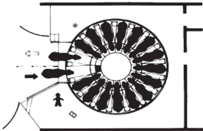
Gambar 20. Layout Mesin Perah Tipe Rotaryy Abreast
