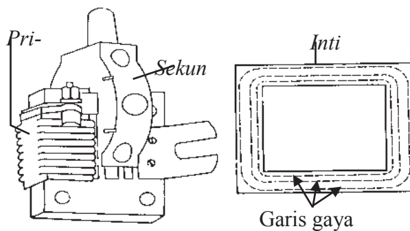
Gambar 2.9: koil inti tertutup
