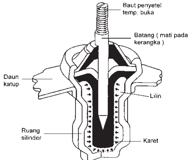
Gambar 4.19: bagian-bagian termostat
