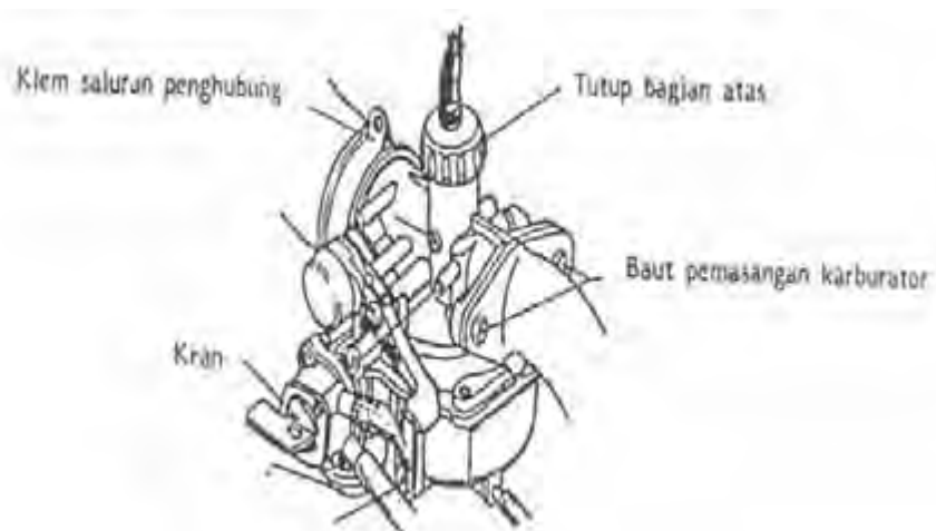
Gambar 5.6: karburator
