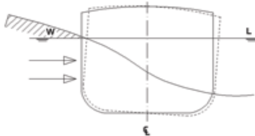
Gambar 3.7 Racking
