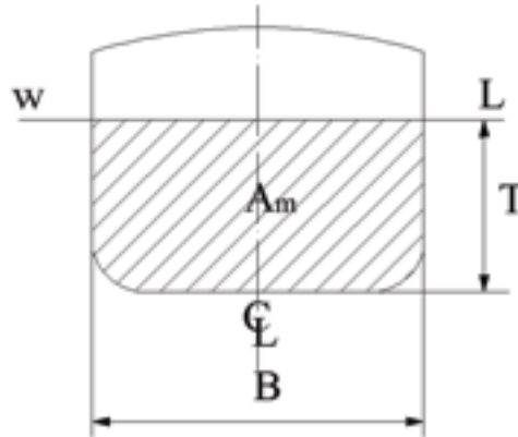
Gambar 5.3 Koefisien Midship
