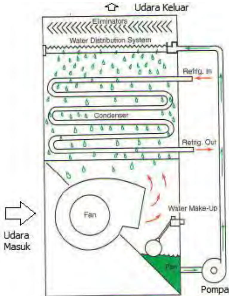
Gambar 2. 23 Evaporative Condenser
