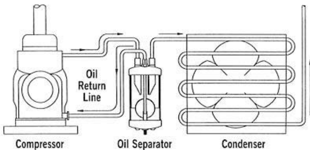
Gambar 2. 37 Oil Separator
