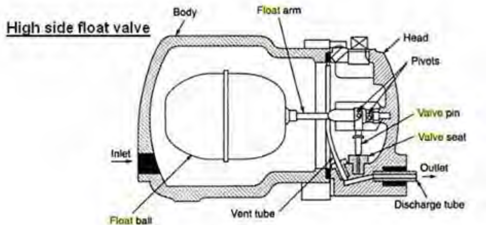
Gambar 2. 34 Float Valve
