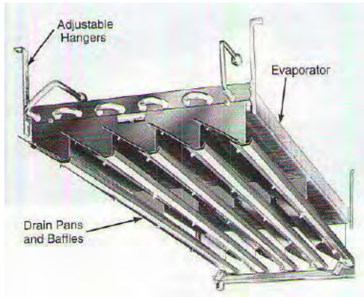
Gambar 2. 25 Non-defrosting Evaporator
