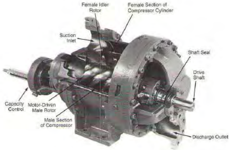
Gambar 2. 18 Screw Compressor
