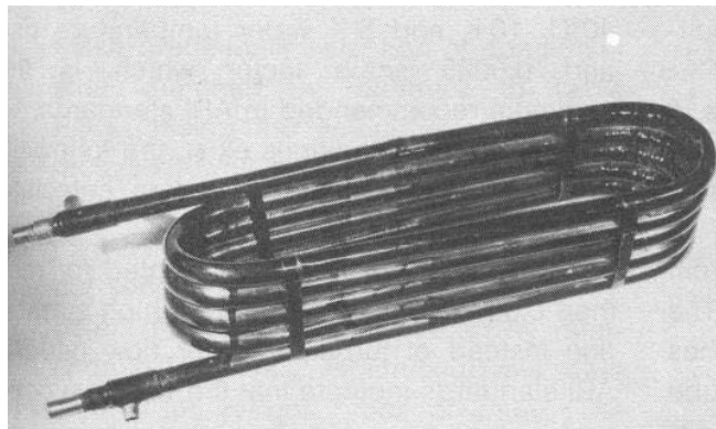
Gambar 4. 28 Tube-in-tube Condenser
