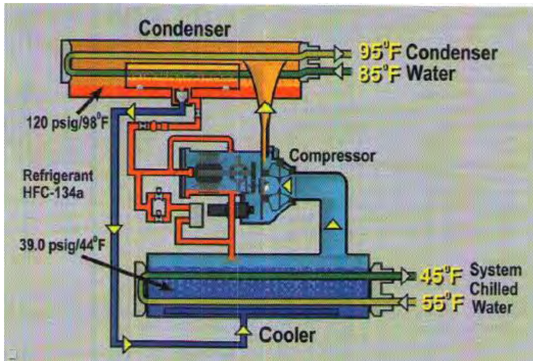
Gambar 2. 19 Centrifugal Compressor
