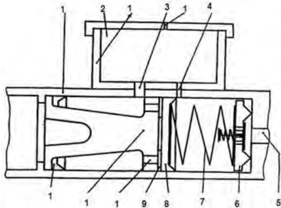
Gambar 2.35. Bagian-bagian silinder master
