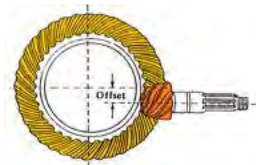
Gambar 4.58. Penggerak roda gigi hypoid (hypoid Bevel Gear)
