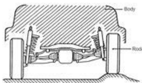
Gambar 5.24. Suspensi Independen
