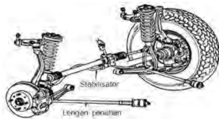
Gambar 5.33. Mac. Pherson Sistem Honda
