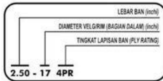
Gambar 7.16. Kode Ban Diagonal
