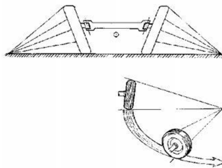
Gambar 6.17. Fungsi camber
