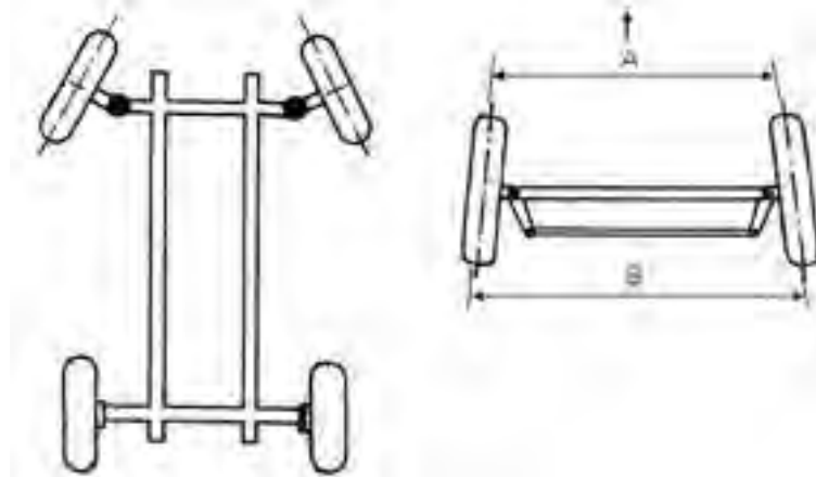
Gambar 6.22. Toe in (positif)
