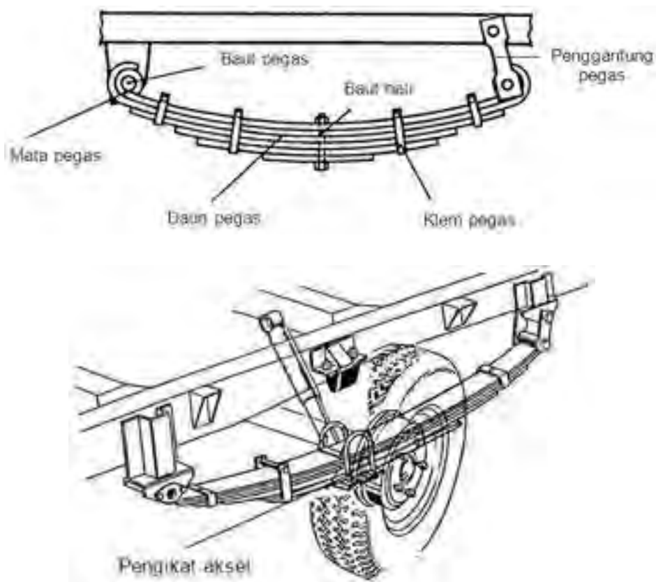
Gambar 5.40. Pegas daun
