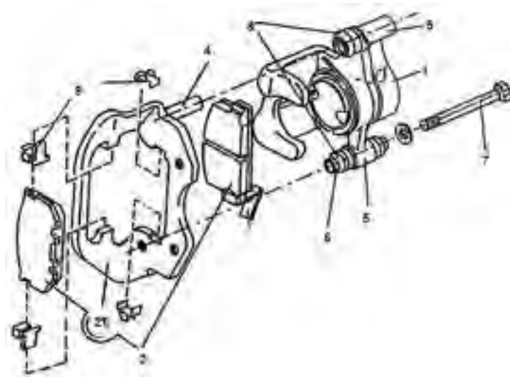
Gambar 2.23.Kaliper Luncur Toyota
