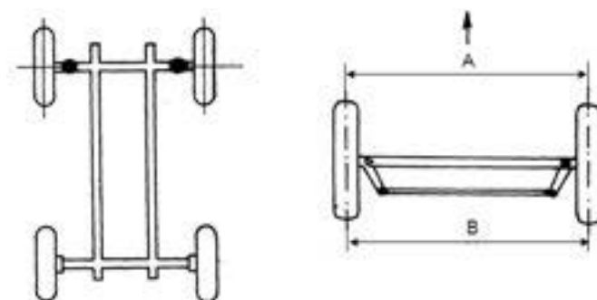
Gambar 6.21. Toe nol
