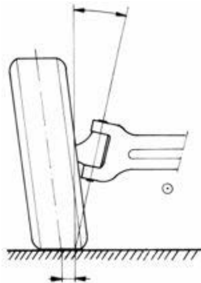
Gambar 6.14. Inklinasi king-pin
