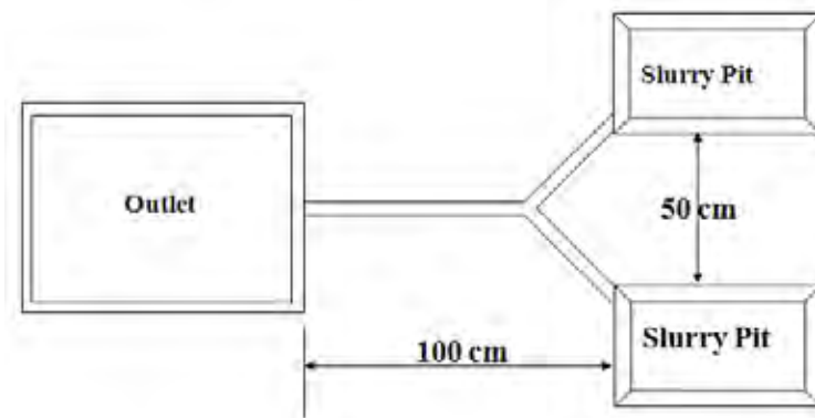
Gambar 149. Gambar denah lubang kompos ( slurry pit )
