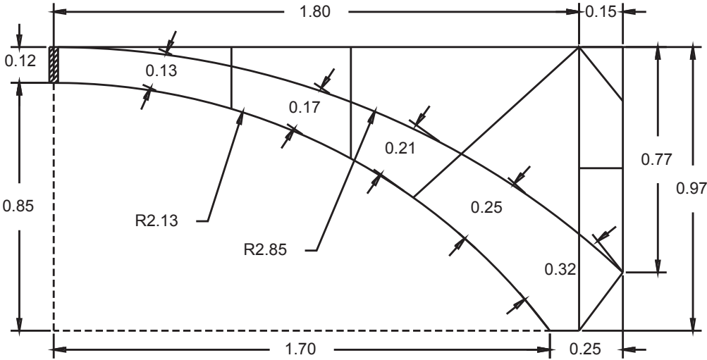
12 m3 biogas Plant Template
