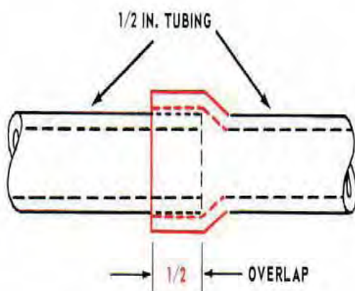
Gambar 5.10 proses swaging
