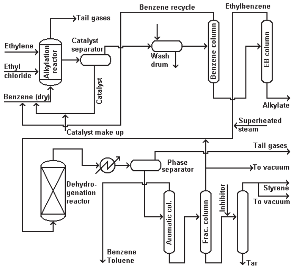
Gambar 16.23 Styrene recovery
