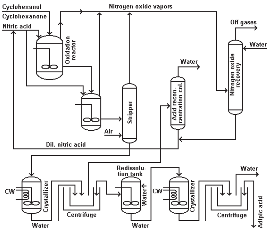
Gambar 16.26 Adipic acid
