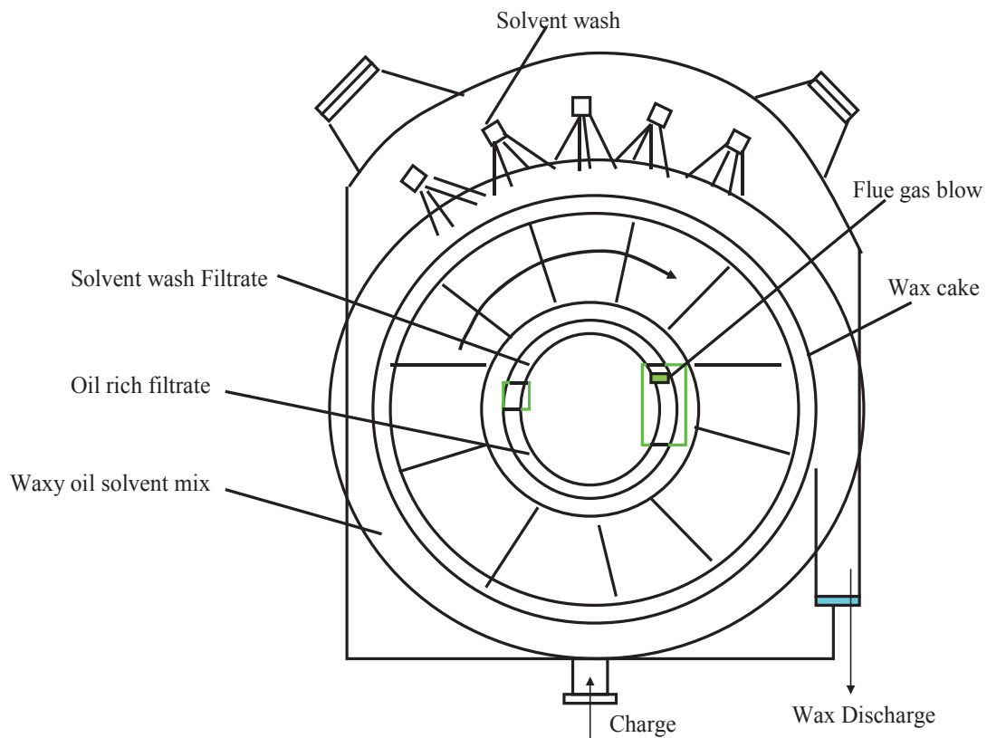
Gambar : 5 - 3 Filter Drum
