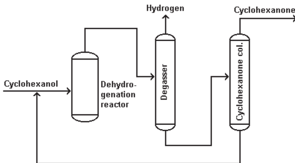
Gambar 16.25 Cyclohexanone
