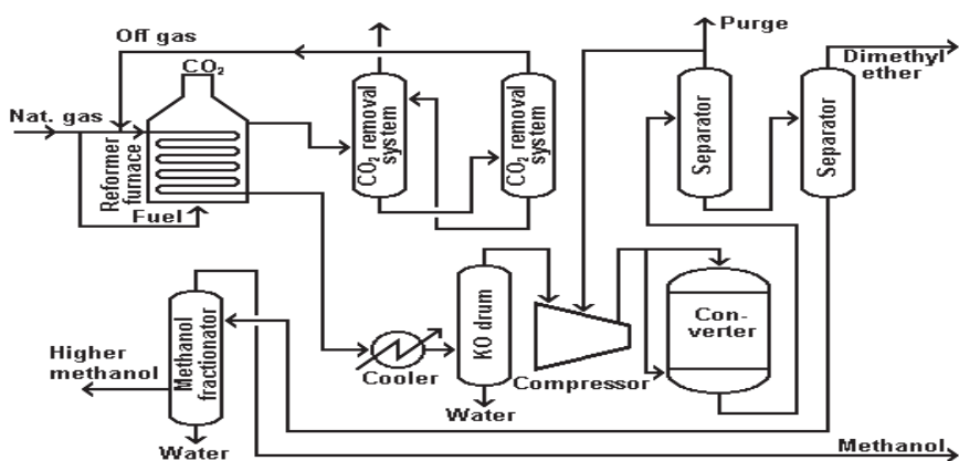
Gambar 16.12 Methanol Plant
