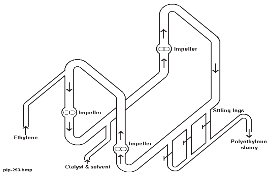
Gambar 16.16 Pipe-Loop Reactor
