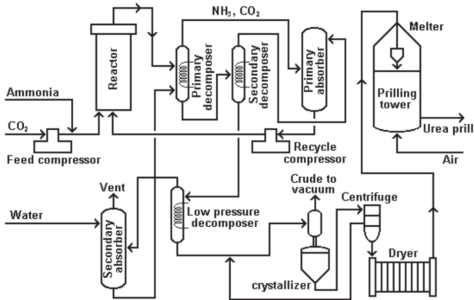
Gambar 16.11 Urea (total recycle)
