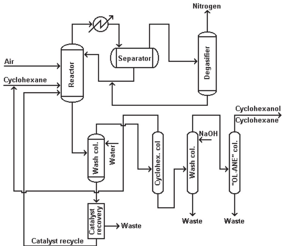
Gambar 16.24 Cyclohexane oxidation
